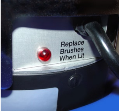
Motor carbon brush wear indicator light alerts the operator to protect the motor.
