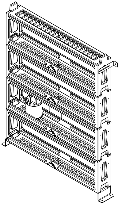
A500 - Stackable Van Shelving System Set
